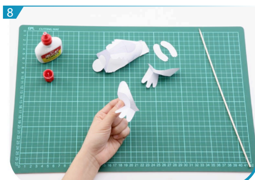
Fold and glue R05 with R06, R07 with R08 to form legs.
